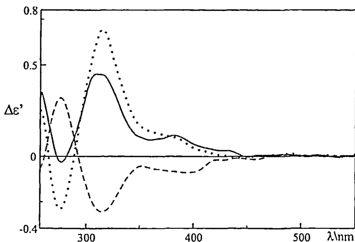
Figure 2: CD spectra of in situ Mo-complexes of compounds 14 R (—), 14 S (---) and 20 (···).
