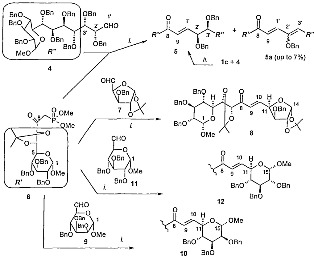
Scheme 2. i . K 2 CO 3 , 18-crown-6, toluene; ii . 12 kbar.
