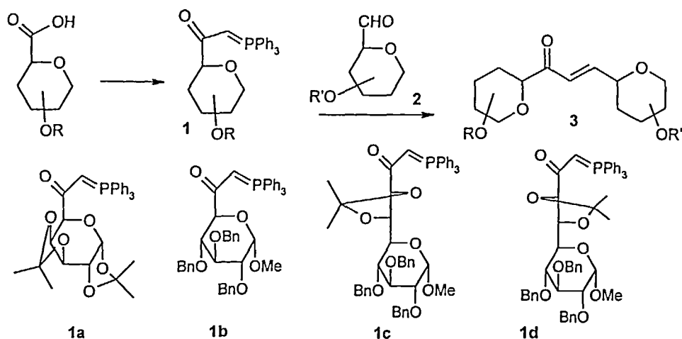
Scheme 1. preparation of higher carbon sugars by application of the Wittig methodology
