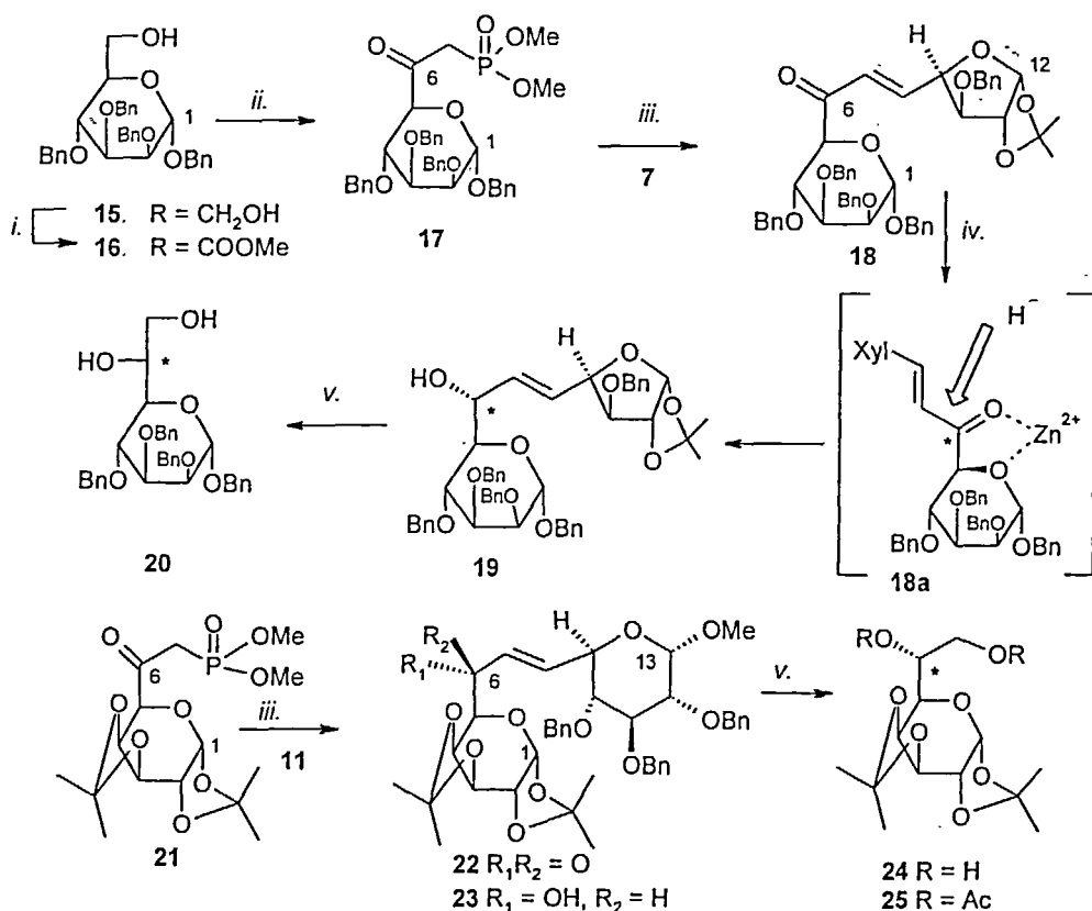
Scheme 4. i. a. Jones' reagent. b. CH 2 N 2 ; ii. 18 C 2 H 5 P(O)(OMe) 2 ; iii. K 2 CO 3 , 18-crown-6, toluene; iv. Zn(BH 4 ) 2 , ether, 0°C; v. a. O 3 b. NaBH 4
